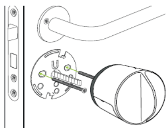
DANALOCK V3 zadná platnička a adaptér
